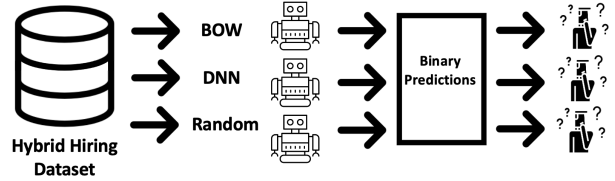
Figure 1: An example hybrid hiring workflow. A candidate dataset is used to train three NLP classifiers, which each outputs recommendations to human decision-makers. We evaluate accuracy and bias of the resulting system.
