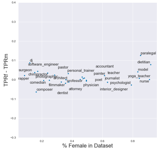
(b) DNN classification bias.
